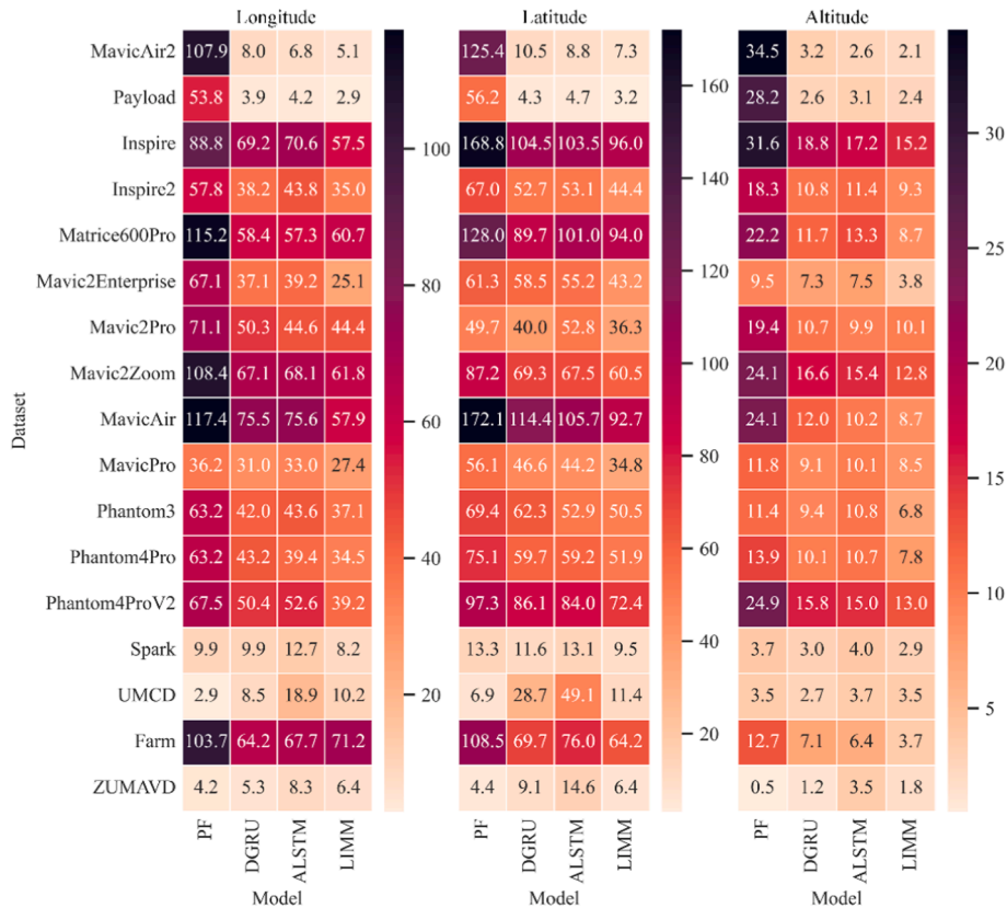
Fig. 7. The comparison of the proposed LIMM model with baselines on MAE (m) in three axes.
