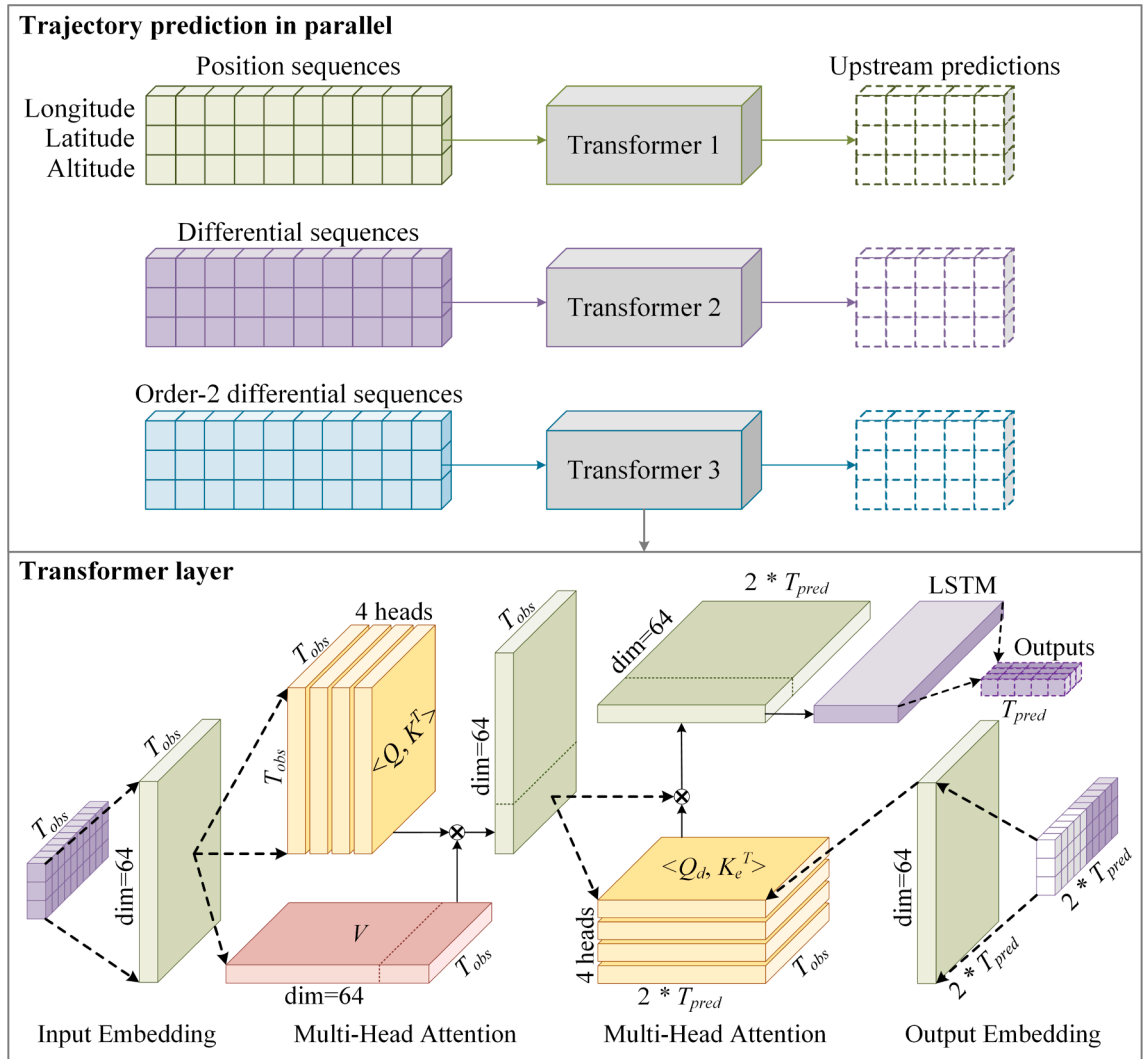
Fig. 3. The framework of differential trajectory prediction in parallel.
